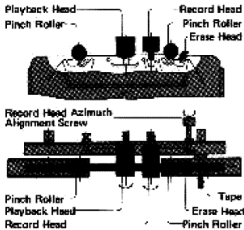
Head Azimuth Alignment
