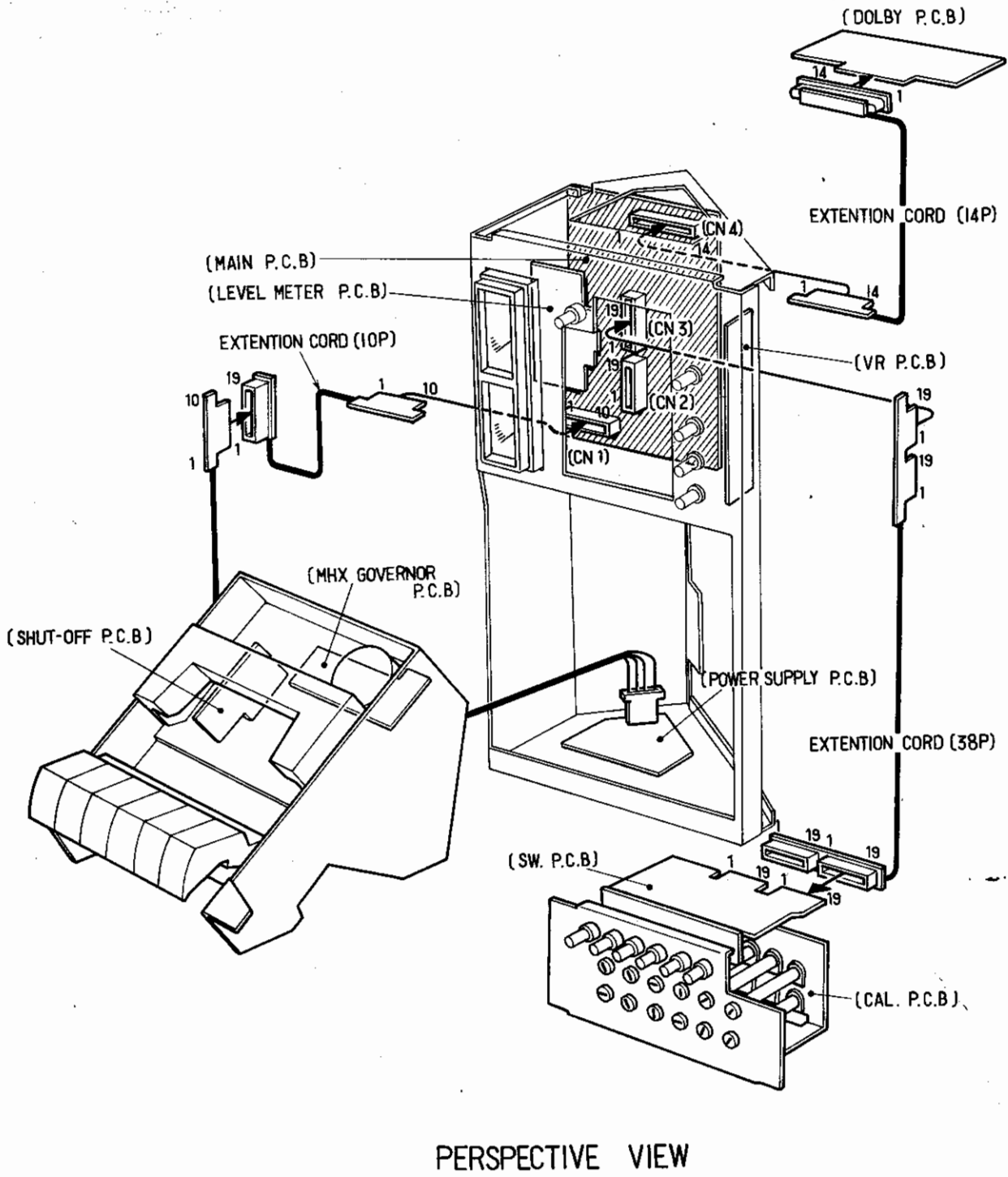
Fig. 4 Extension Cord Connection
