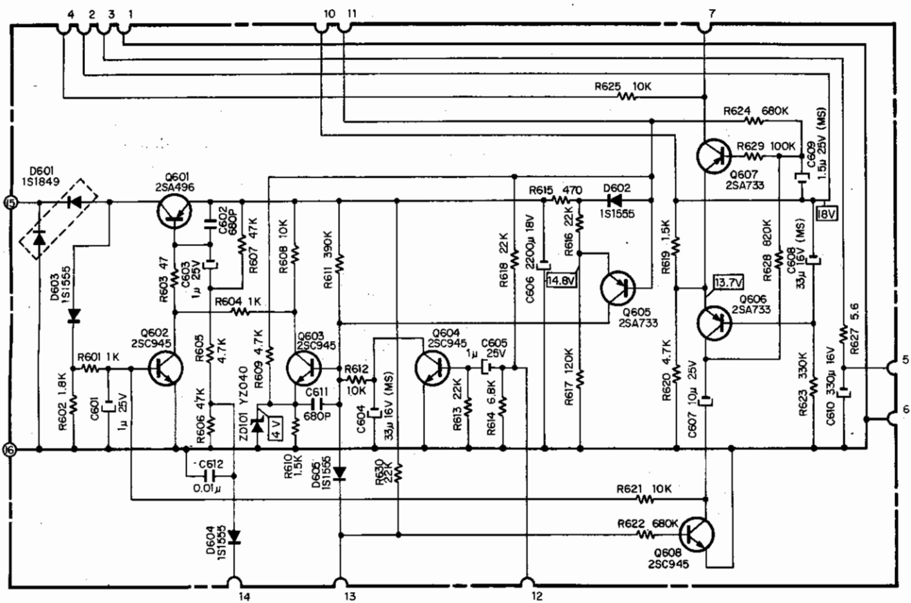
Fig. 2. 3. 1 Shut-off Circuit
